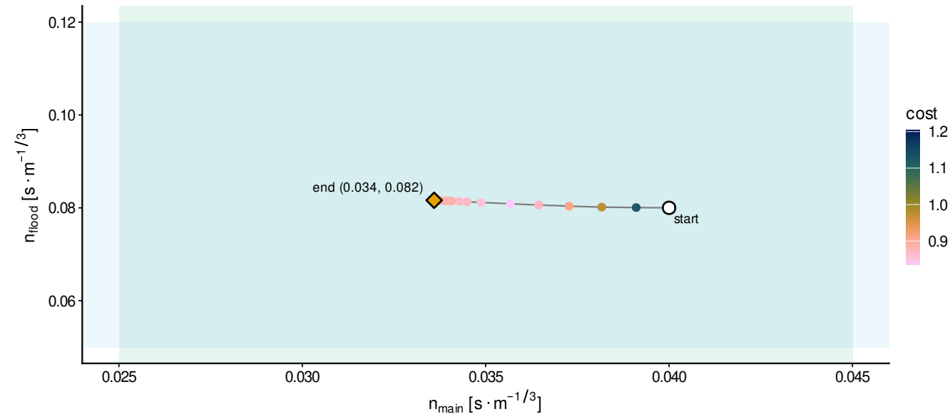
(b) objective convergence
