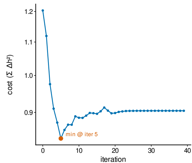
(b) objective convergence
