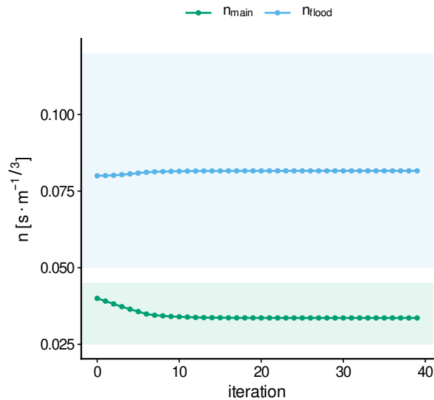
(c) parameters vs iteration
