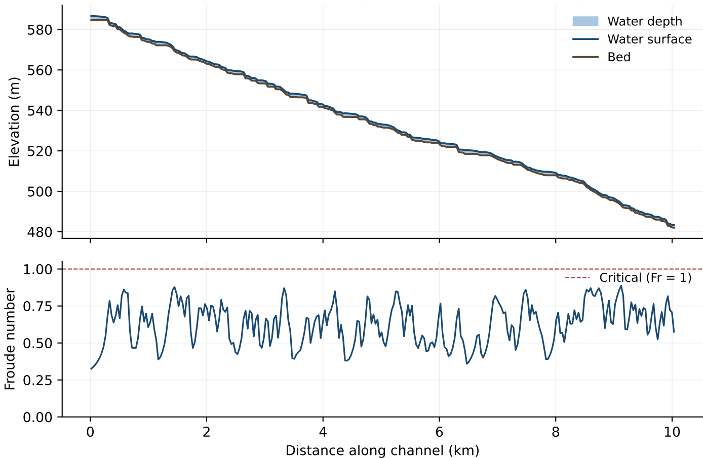
Río Maule reach — hydroflux-solver-1d steady state ( n = 288 , dx = 34.9 m, q = 3 m 2 /s, n = 0.04 )
