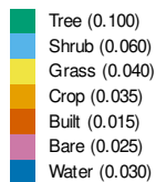
Class (n)
