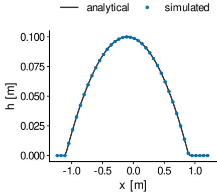
(c) Thacker oscillation ( t = T/2 )
