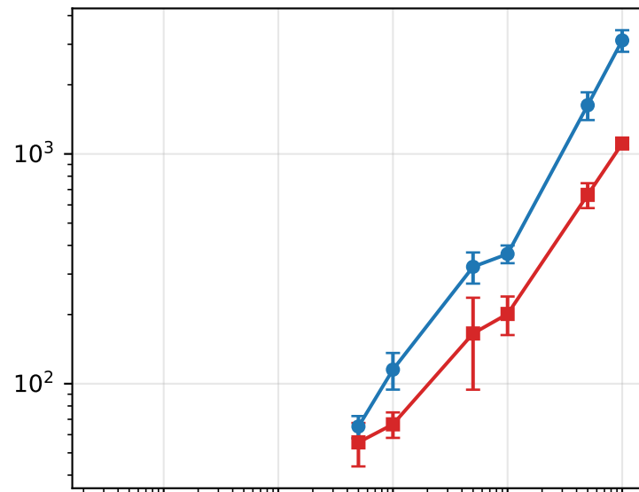
LightGBM — Classification
