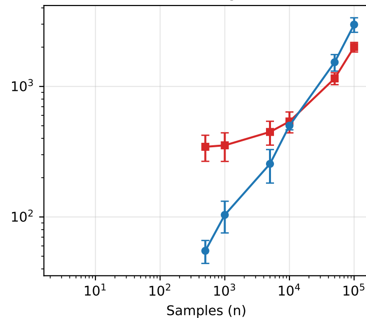
CatBoost — Regression
