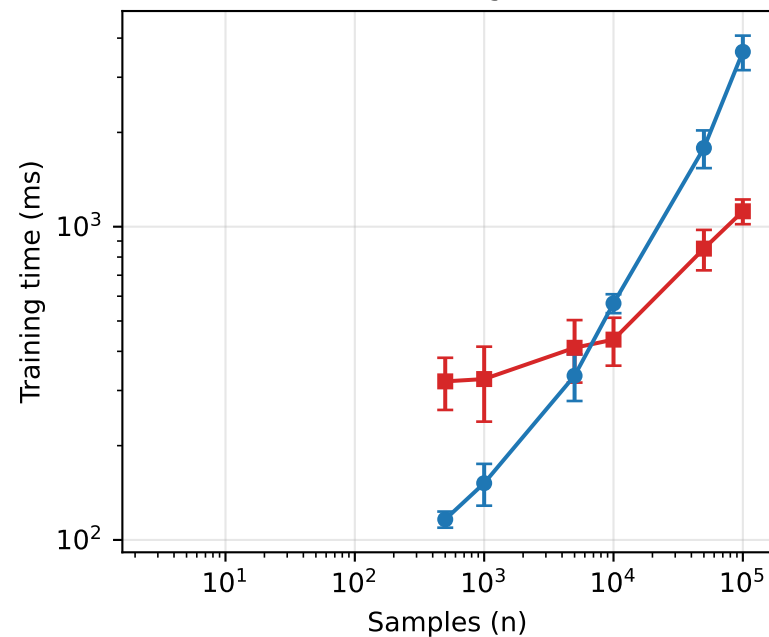
XGBoost — Regression
