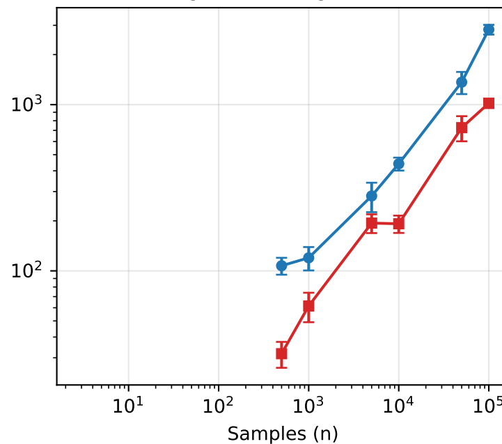
LightGBM — Regression
