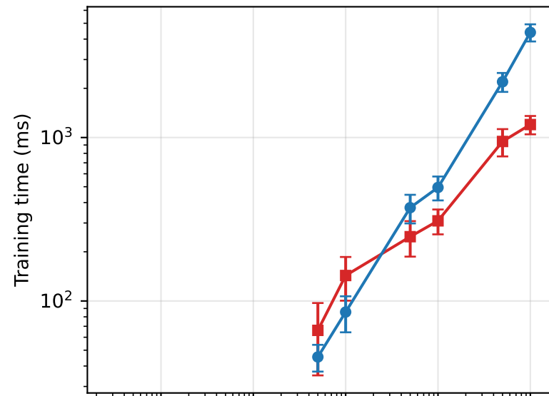
XGBoost — Classification
