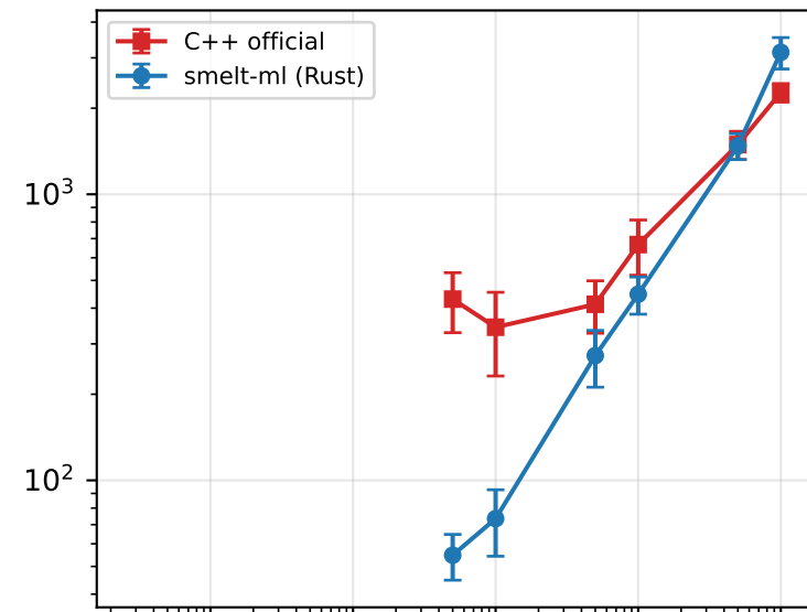
CatBoost — Classification
