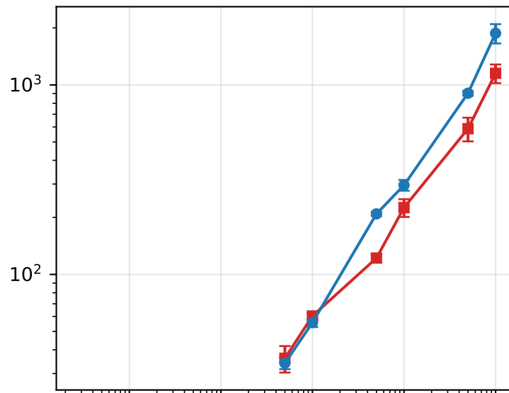
LightGBM — Regression
