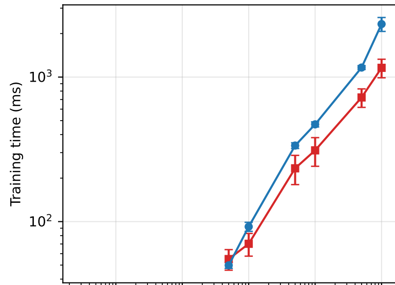
XGBoost — Regression
