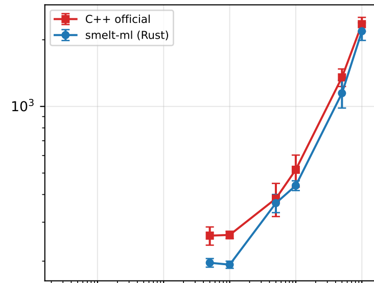
CatBoost — Regression
