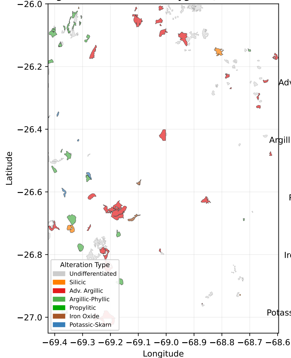
(b) Region III — Alteration Polygons (Atlas Metalífero)
