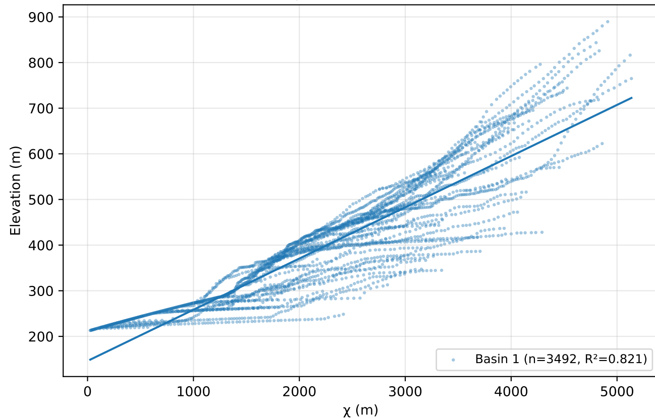
Smugglers Notch — elevation vs \chi per basin (Perron & Royden 2013 linearisation test)
