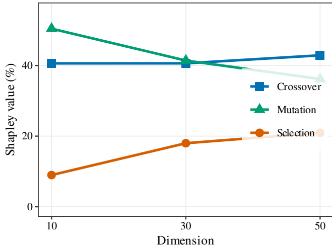
GA: Operator attribution vs dimension
