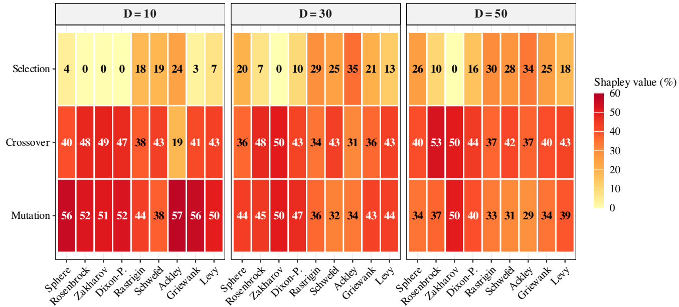
GA: Exact Shapley values by function and dimension
