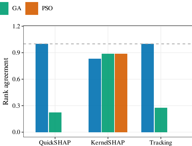
Accuracy: rank agreement vs Exact
