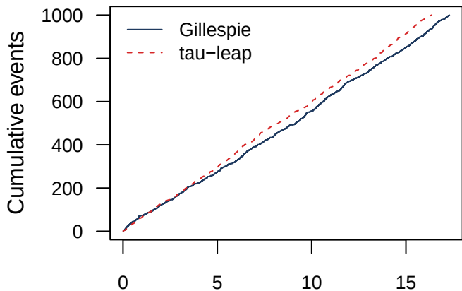
Cumulative count: both algorithms
