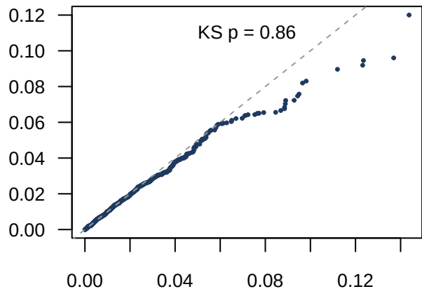
QQ-plot of inter-event times
