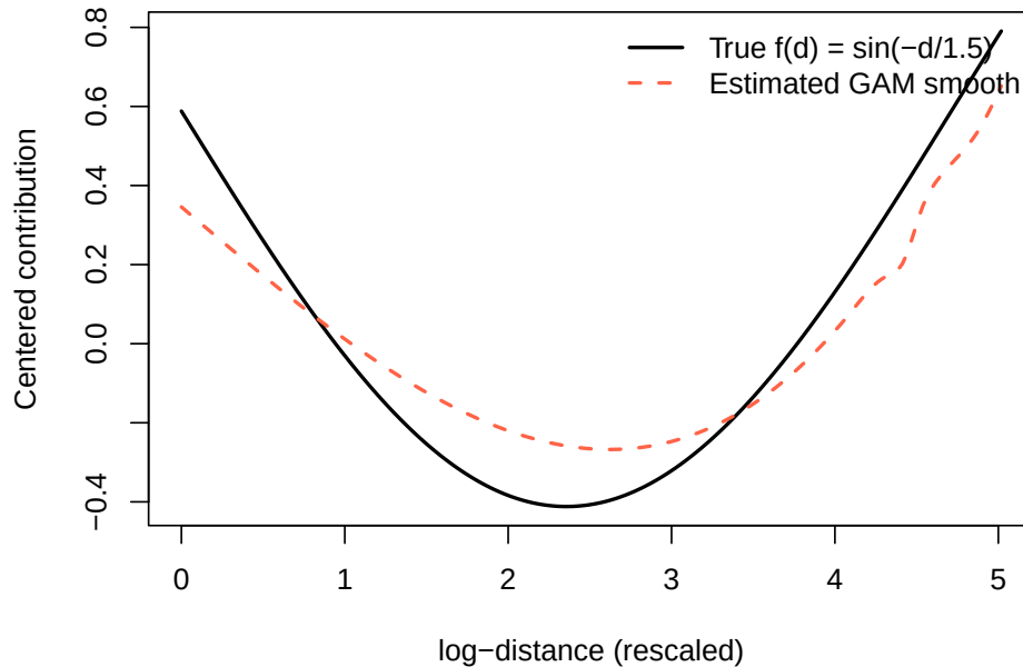
Figure 7: Experiment 2: estimated GAM smooth (dashed) vs. the true sinusoidal effect (solid). Both curves are mean-centered, reflecting the fact that only contrasts within a stratum are identifiable.
