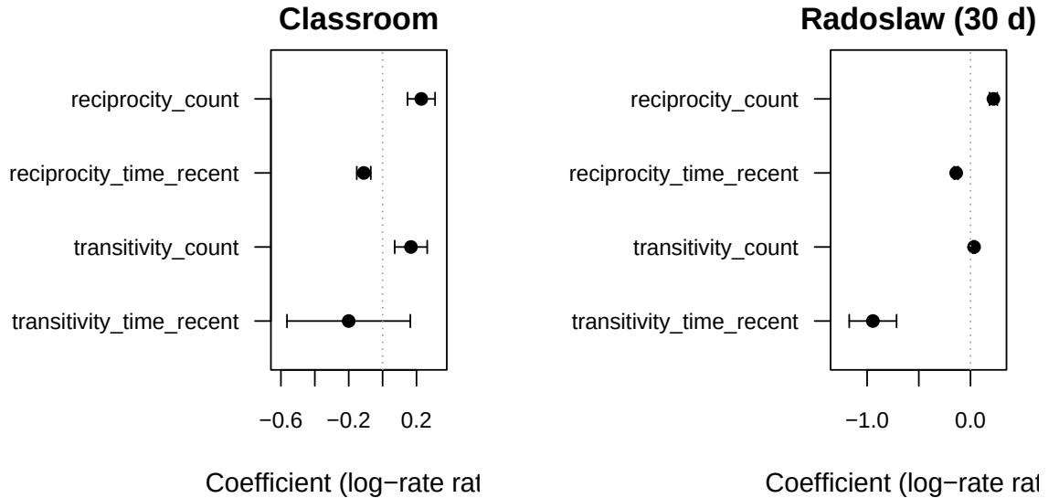
Figure 2: Coefficient estimates and 95% Wald intervals for the four endogenous statistics fitted on Classroom (left) and a 30-day slice of Radoslaw (right). Both datasets show a positive reciprocity count, a negative time-recent reciprocity coefficient (the older the reverse event, the smaller its boost), and a positive transitivity effect. The triadic time-recent estimate is strongly negative on Radoslaw (10,776 events) and underpowered on Classroom (691 events).
