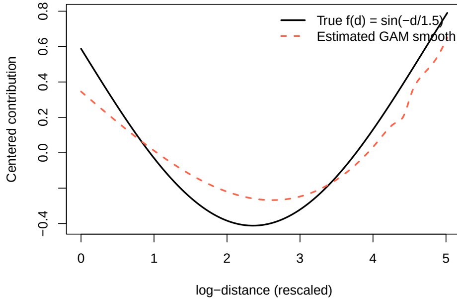
Figure 1: Experiment 2: estimated GAM smooth (dashed) vs. the true sinusoidal effect (solid). Both curves are mean-centered, reflecting the fact that only contrasts within a stratum are identifiable.
