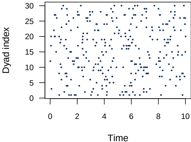
Plain Gillespie: 300 events, 6 actors
