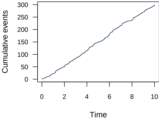
Mean rate = 30.0 events / unit time
