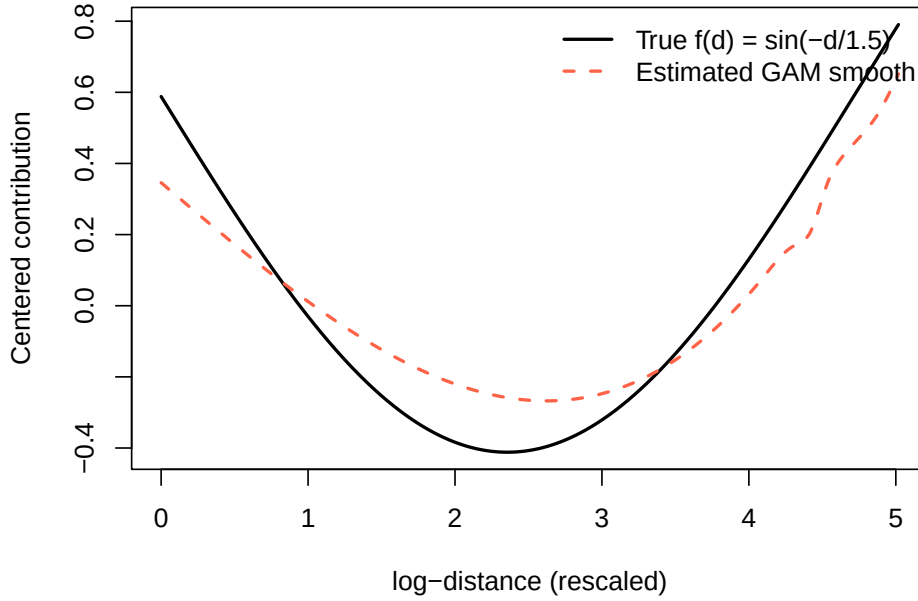
Figure 7: Experiment 2: estimated GAM smooth (dashed) vs. the true sinusoidal effect (solid). Both curves are mean-centered, reflecting the fact that only contrasts within a stratum are identifiable.
