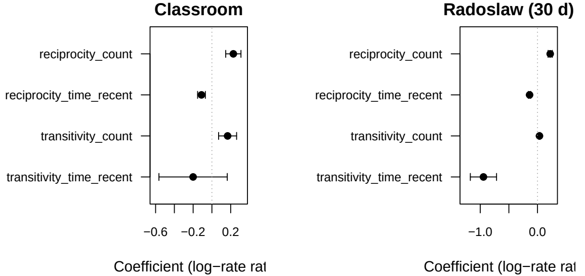
Figure 13: Coefficient estimates and 95% Wald intervals for the four endogenous statistics fitted on Classroom (left) and a 30-day slice of Radoslaw (right). Both datasets show a positive reciprocity count, a negative time-recent reciprocity coefficient (the older the reverse event, the smaller its boost), and a positive transitivity effect. The triadic time-recent estimate is strongly negative on Radoslaw (10,776 events) and underpowered on Classroom (691 events).
