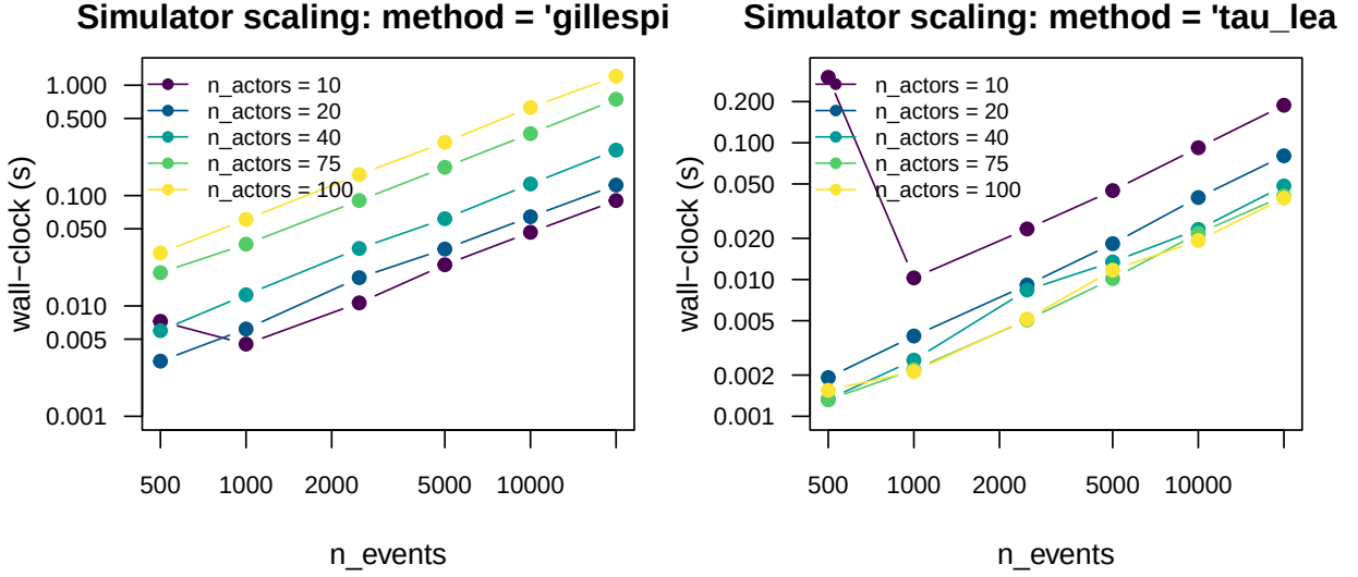
Figure 8: Simulator wall-clock vs n_{\text{events}} on log-log axes, for each n_{\text{actors}} . The Gillespie path (left) is near-linear in n_{\text{events}} with a multiplicative n_{\text{actors}} factor; the \tau -leap path (right) is also near-linear in n_{\text{events}} but decreases with n_{\text{actors}} (the per-step Poisson-sampling cost is amortised over many dyads).
