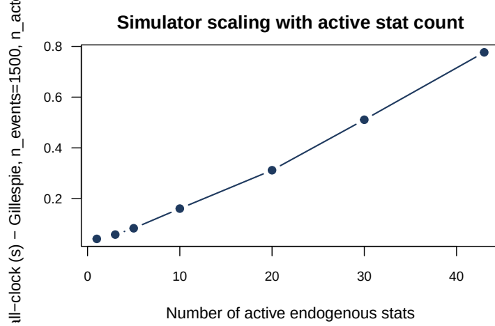
Figure 9: Simulator wall-clock scales near-linearly with the number of active endogenous statistics.
