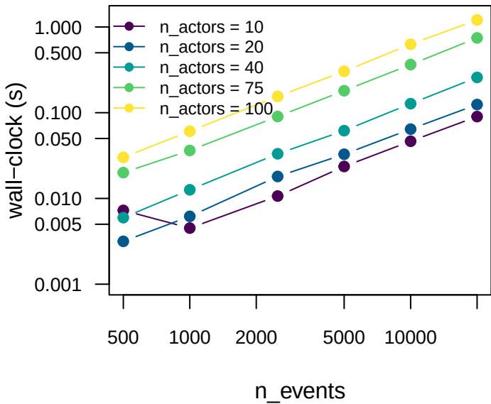
Simulator scaling: method = 'gillespi'
