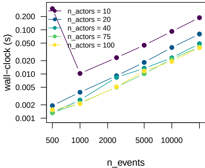
Simulator scaling: method = 'tau_lea'
