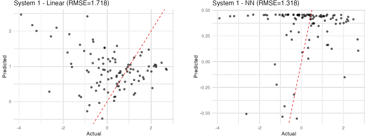
Figure 4: Predicted vs. actual on the System 1 test set. Left: Linear. Right: NN.
