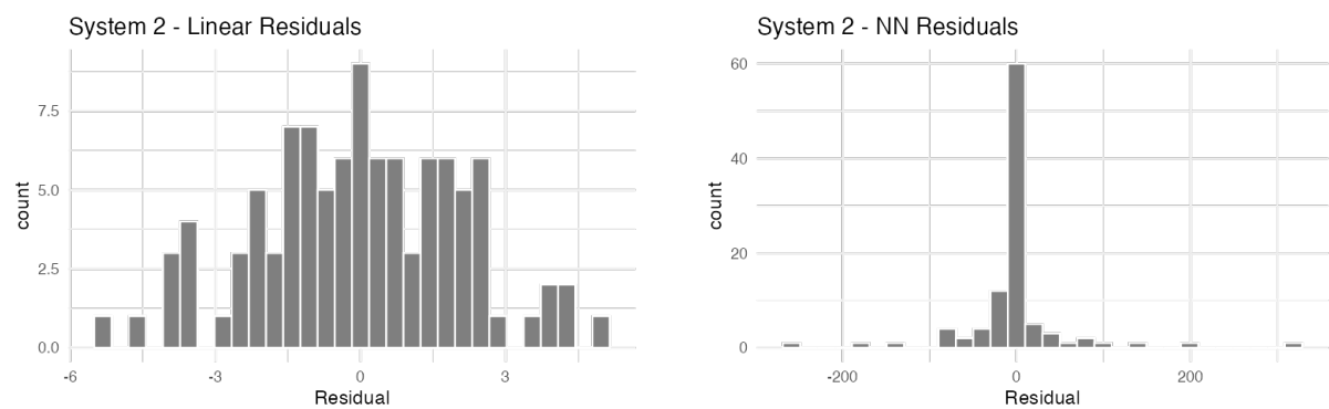
Figure 3: System 2 residual histograms on test set. Left: Linear. Right: NN.
