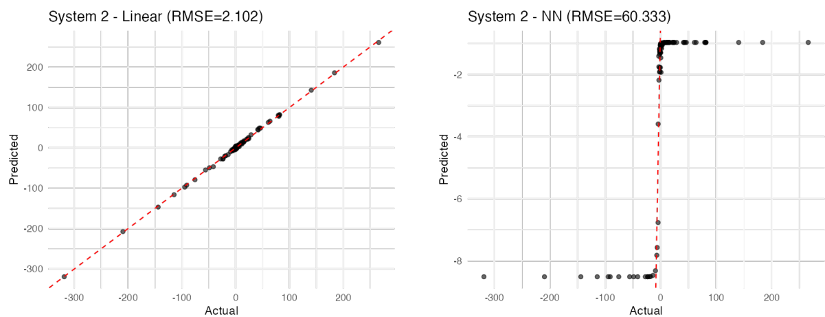
Figure 1: System 2 predicted vs. actual on test set. Left: Linear. Right: NN.
