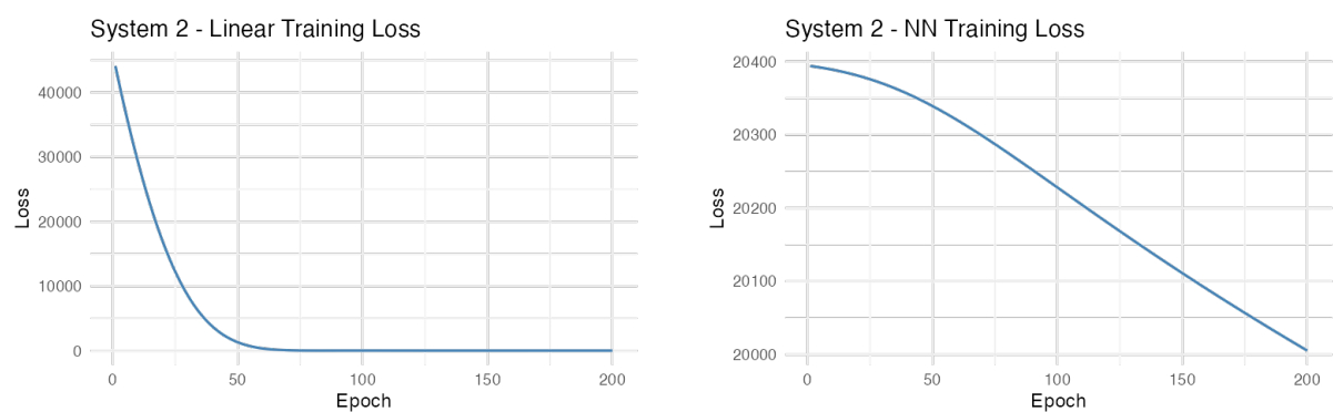
Figure 2: System 2 training loss curves (Adam). Left: Linear. Right: NN.
