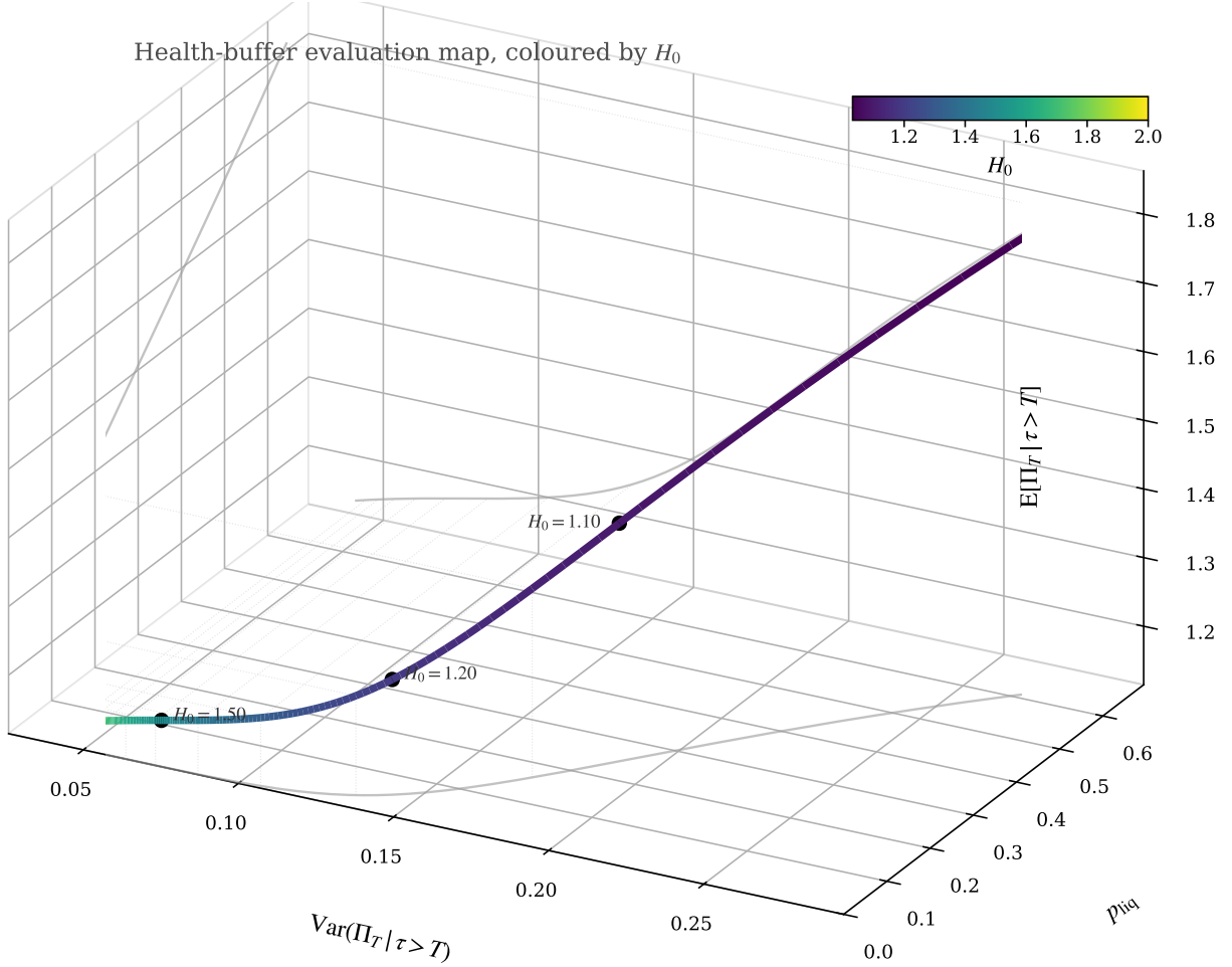
Figure 1: Health-buffer evaluation map for the calibrated long-WETH/short-WBTC benchmark in Table 2. Axes: x = \text{Var}(\Pi_T | \tau > T) , y = p_{\text{liq}} = 1 - p_{\text{surv}} , and z = E[\Pi_T | \tau > T] . The curve is parametrised and coloured by H_0 \in [1.031, 2.000] ; labelled points identify representative initial health factors. Grey curves are orthogonal guides on the coordinate planes.
