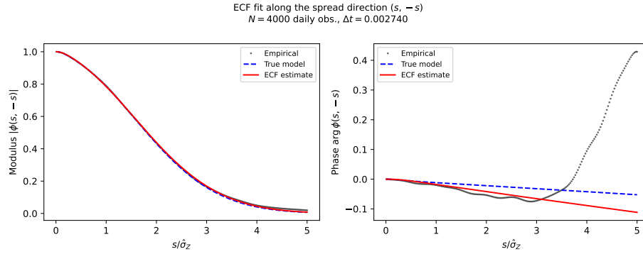
Figure 1: Shape-only ECF fit along the spread direction ( s, -s ) for N = 4,000 synthetic daily observations from a residual law with zero expected log drift. Left: modulus |\phi(s, -s)| ; right: phase \arg \phi(s, -s) . Dots: empirical CF \hat{\phi}_N ; dashed: true residual-law CF; solid red: shape-only ECF estimate. Agreement in this liquidation-relevant direction is a shape diagnostic; it does not validate the directional-drift forecast. Script optimal_long_short/job_runners/calibrate_kou.py .
