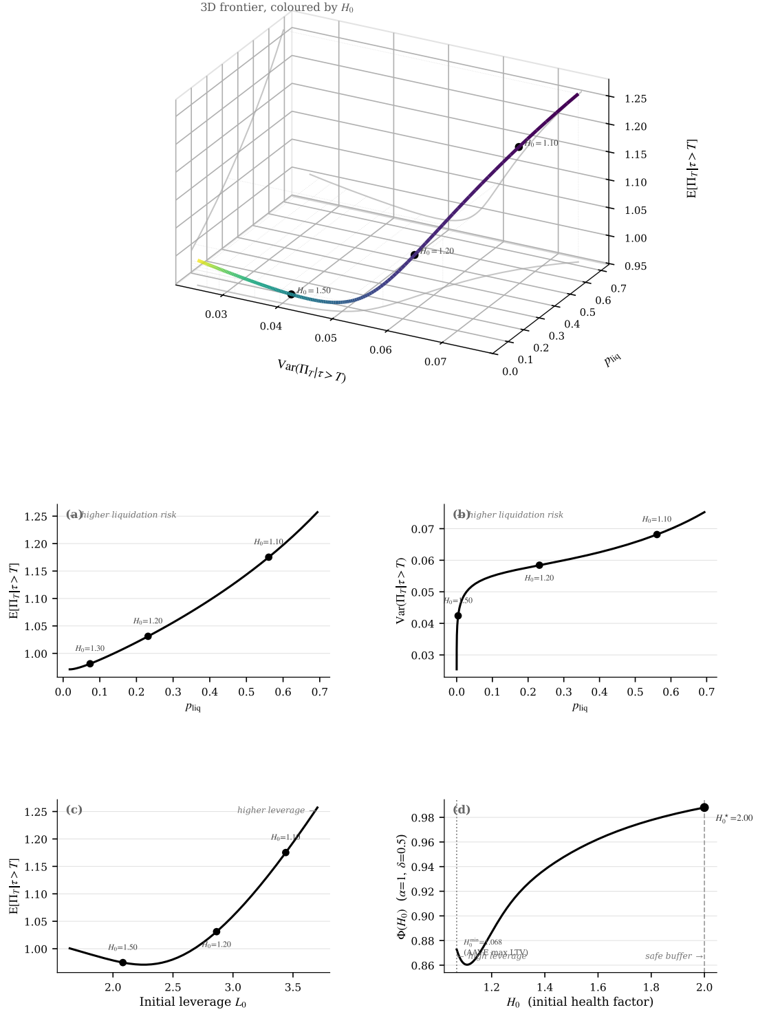
Figure 2: Mean–variance–liquidity frontier of \Pi_T | \{\tau > T\} for the benchmark parametrisation. Axes: x = \text{Var}(\Pi_T | \tau > T) , y = p_\ell = 1 - p_{\text{surv}} , z = E[\Pi_T | \tau > T] (vertical). The curve is parametrised by H_0 \in [1.068, 2.000] ; decreasing H_0 moves the curve toward higher variance and higher p_\ell , while the conditional mean becomes U-shaped near the liquidation boundary. Grey projections on the three coordinate planes recover the pairwise two-dimensional tradeoffs; panel (a) plots the increasing efficient branch of the mean–liquidity projection. Script jobs/frontier_analysis.py .
