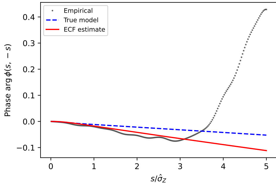
ECF fit along the spread direction ( s, -s ) N = 4000 daily obs., \Delta t = 0.002740
