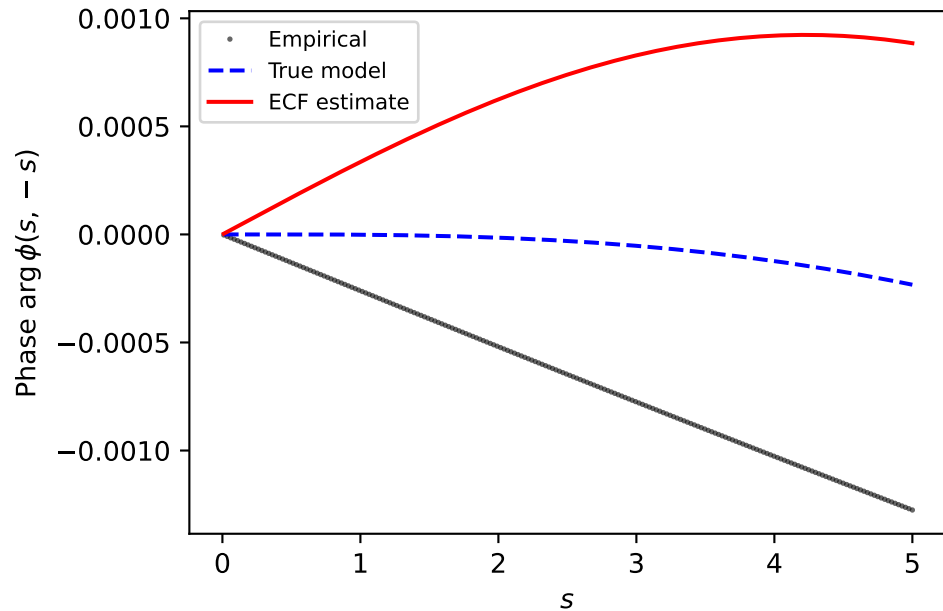
ECF fit along the spread direction ( s, -s ) N = 4000 daily obs., \Delta t = 1/252
