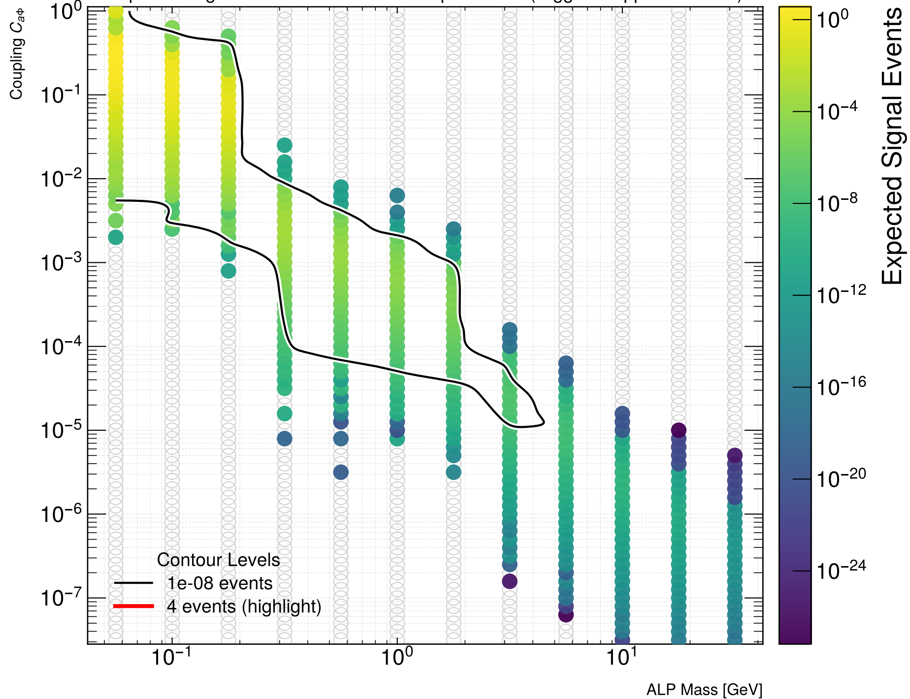
Expected Signal Events for Fermion-Coupled ALPs (Higgs and pp Production)
