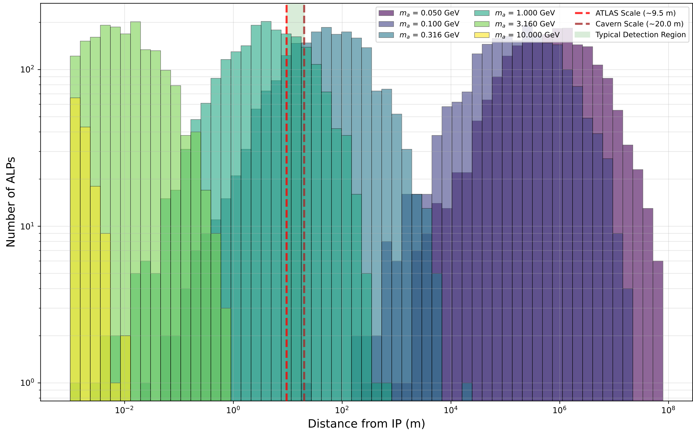
ALP Distance from IP Distributions: All Masses ( C_{a\phi} = 0.001000 )
