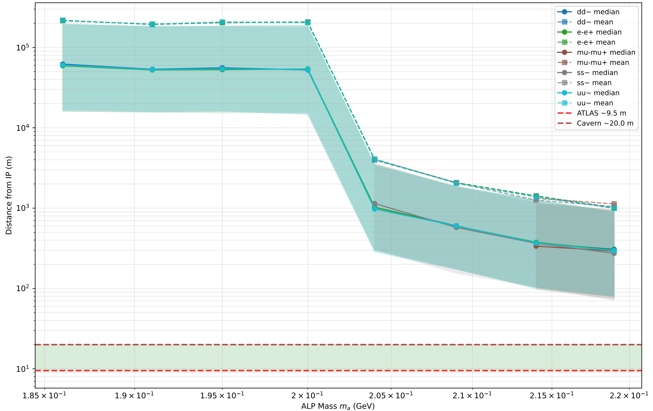
ALP Distance from IP Statistics vs Mass (CaPhi = 0.001000)
