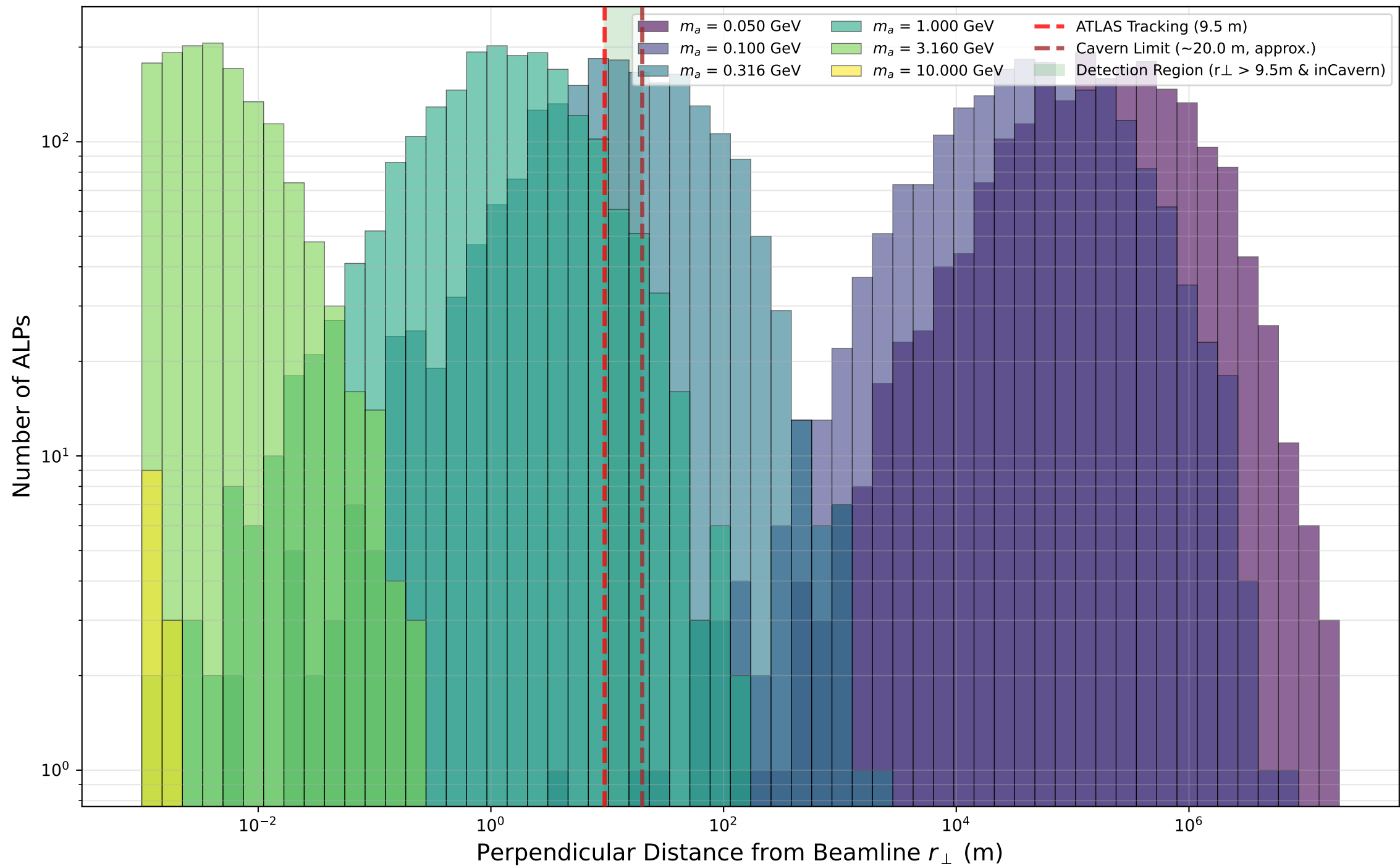
ALP r_{\perp} Distributions: All Masses (Perp. Distance from Beamline, C_{a\phi} = 0.001000 )
