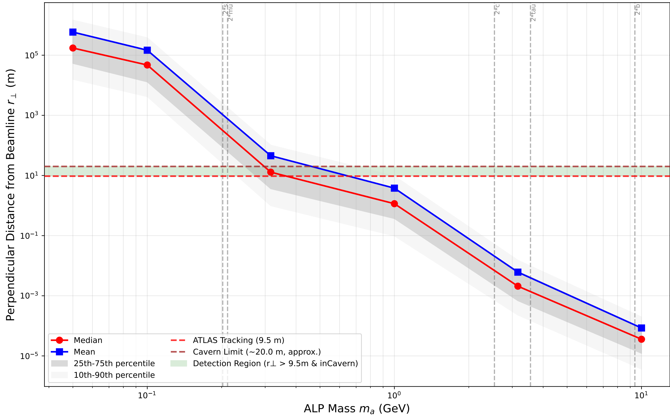
ALP r_{\perp} Statistics vs Mass (Perp. Distance from Beamline, C_{a\phi} = 0.001000 )
