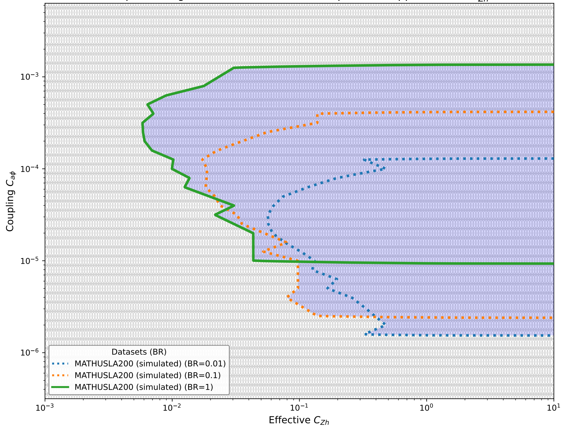
Simulated MATHUSLA200 Expected Signal Events for Fermion-Coupled ALPs, pp \rightarrow H \rightarrow Za , C_{Zh}^{eff} \in [0.001, 10] , m_a = 1 GeV
