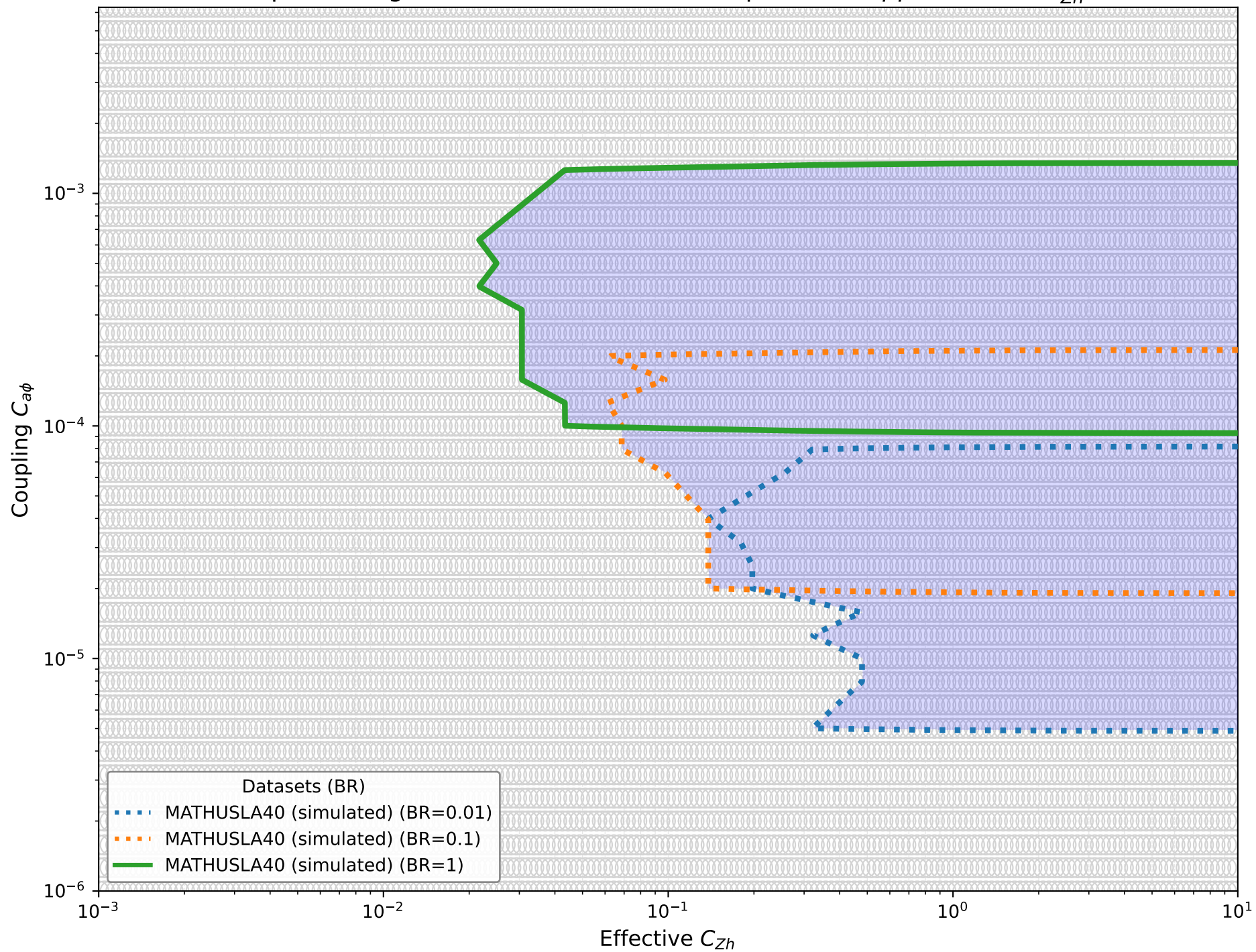
Simulated MATHUSLA40 Expected Signal Events for Fermion-Coupled ALPs, pp \rightarrow H \rightarrow Za , C_{Zh}^{\text{eff}} \in [0.001, 10] , m_a = 1 GeV
