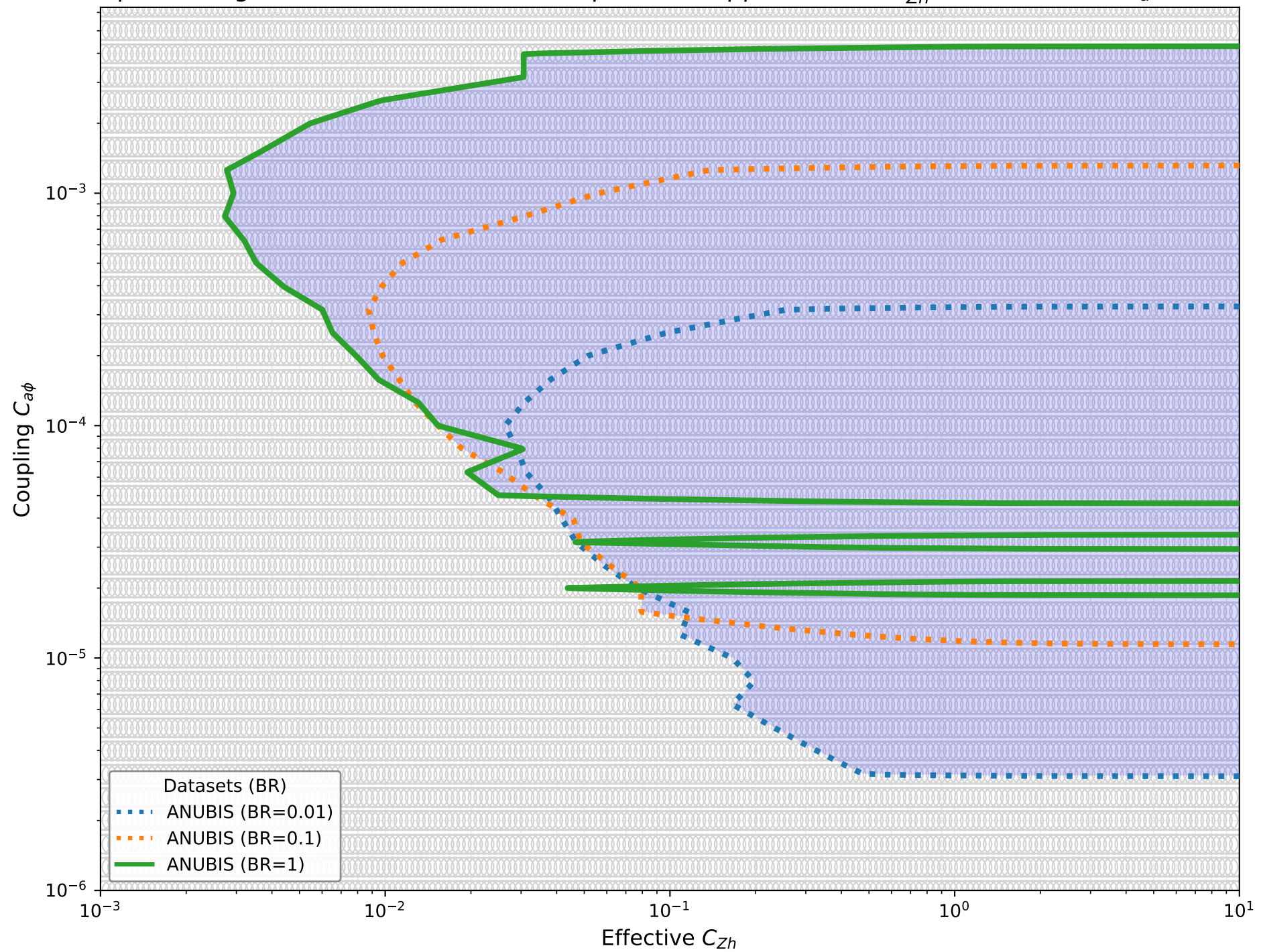
Expected Signal Events for Fermion-Coupled ALPs, pp \rightarrow H \rightarrow Za , C_{Zh}^{\text{eff}} \in [0.001, 10] , m_a = 1 \text{ GeV}
