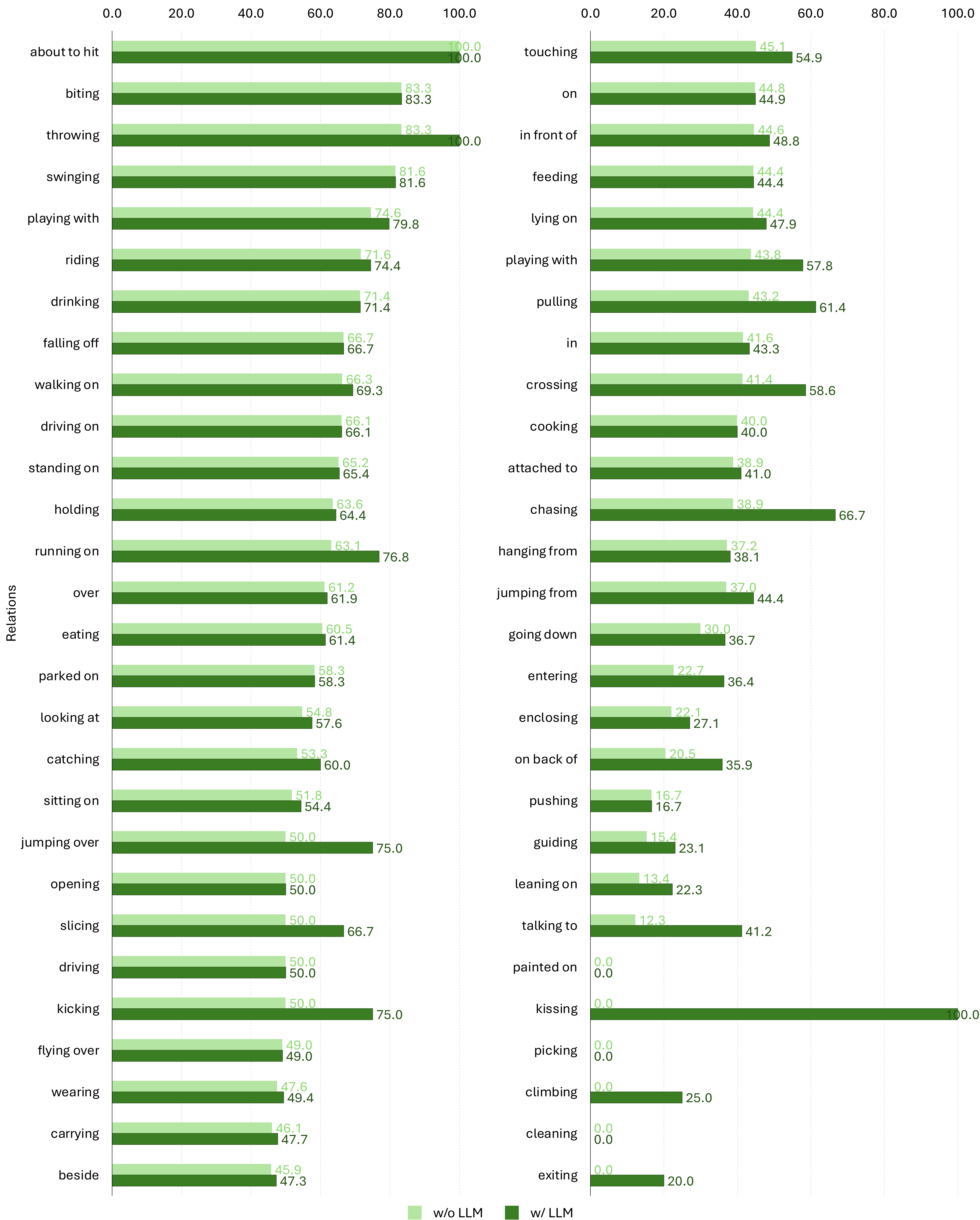
Predicate-wise R@100 results on PSG dataset
