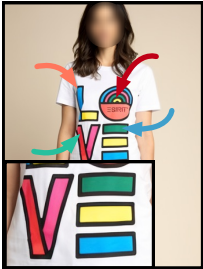
with \mathcal{L}_{\text{leffa}}
