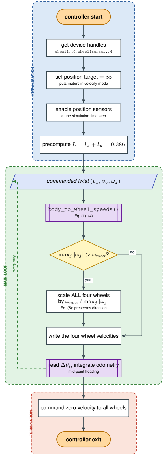
Figure 2: Mecanum base controller (Phase A). The initialisation band holds everything computable once, including the Webots idiom of setting a motor’s position target to infinity to obtain velocity control. The saturation test is the only branch in the loop, and it scales all four wheels together so that a speed limit costs magnitude and never direction. The termination band exists because a controller that exits without zeroing the wheels leaves the base coasting into the next run.
