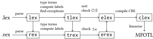
Figure 14: Structure of the Lex compiler
