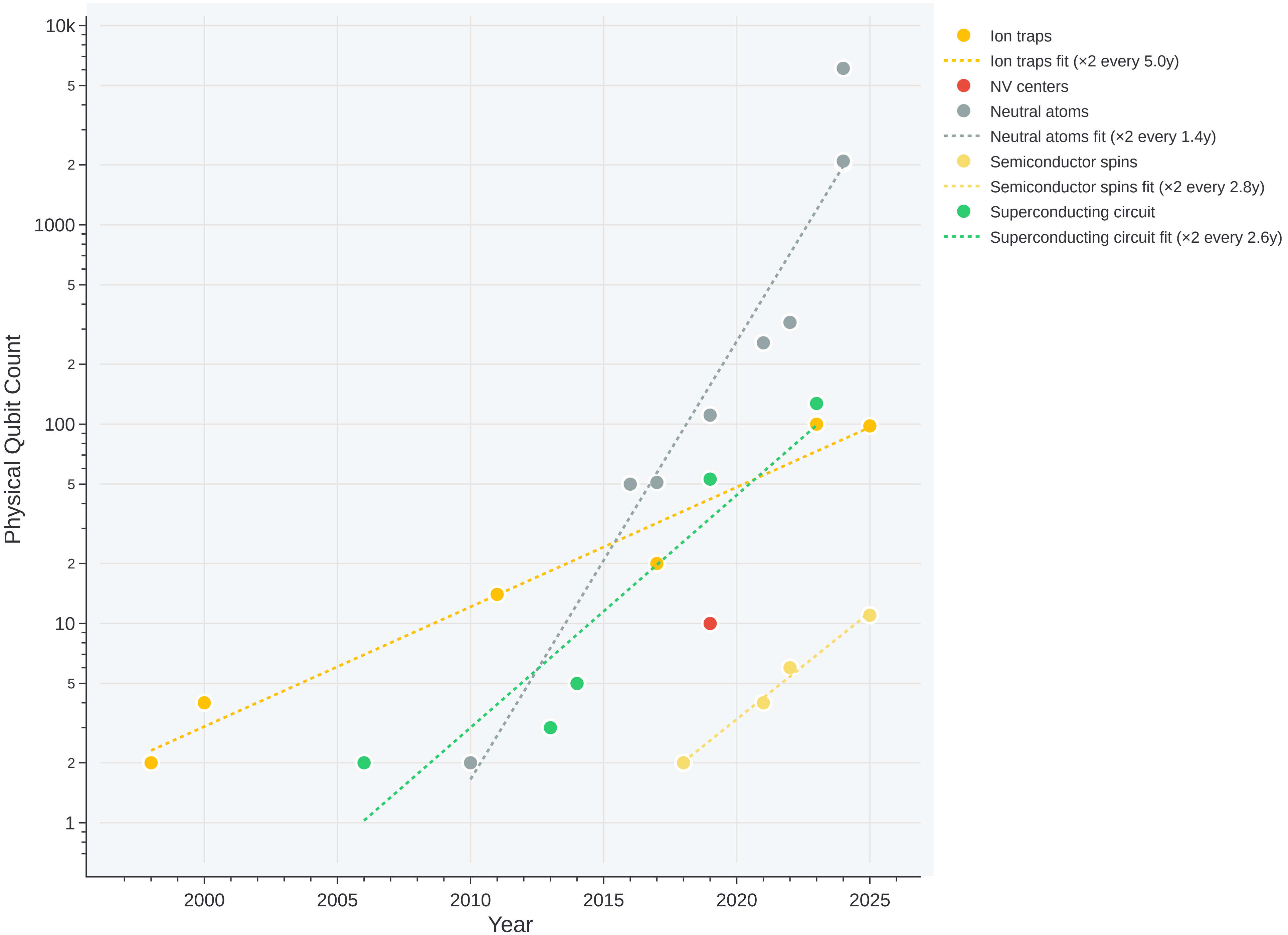
Physical Qubit Count Evolution
