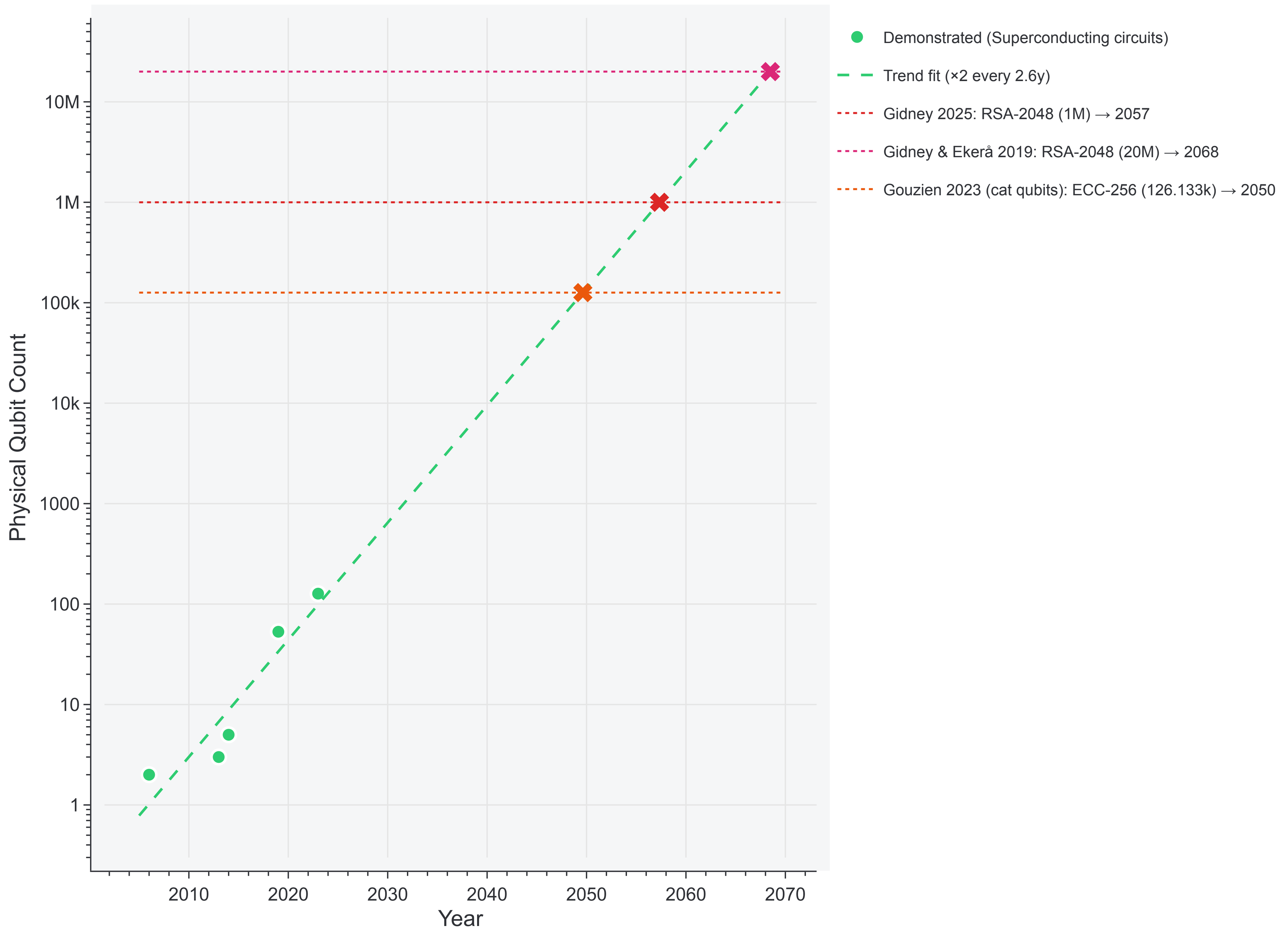
Superconducting circuits: physical qubit count vs. requirements
