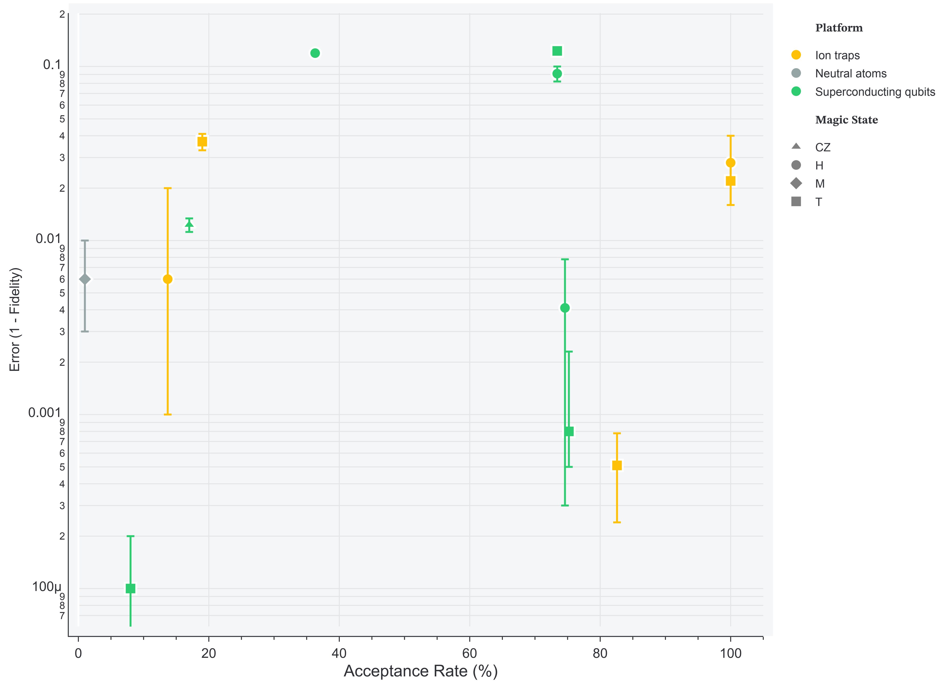
Magic State Preparation: Error vs Acceptance Rate
