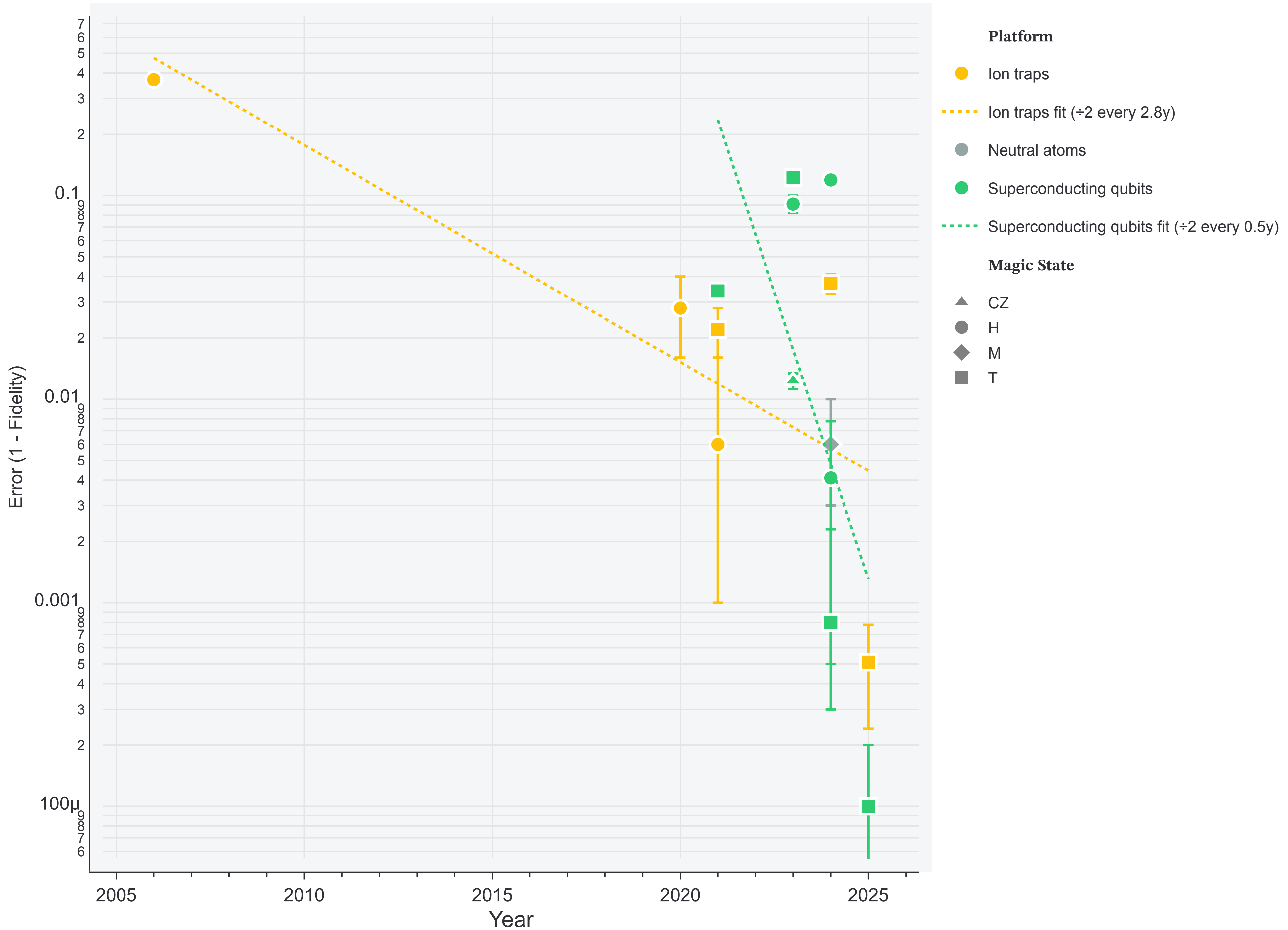
Magic State Error Evolution Over Time
