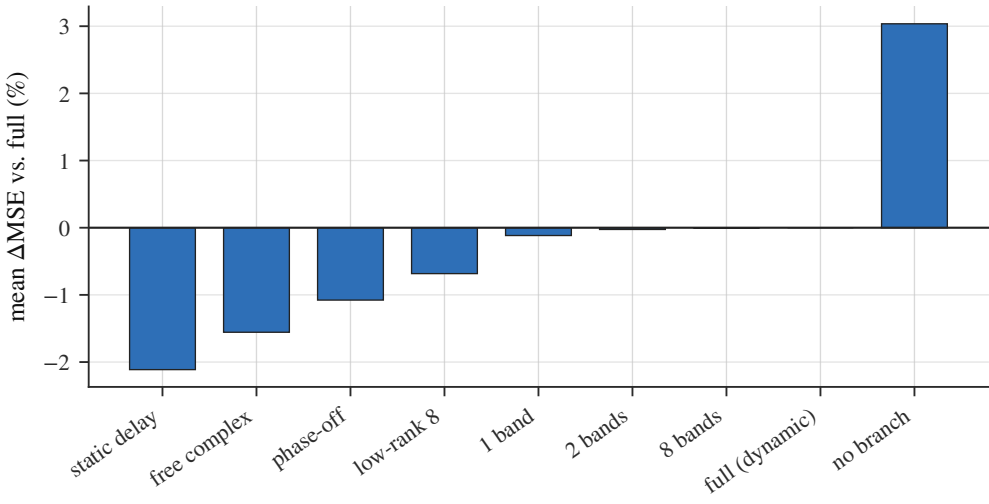
Ablation: change relative to the full model (5 datasets)
