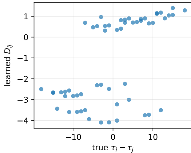
delay recovery ( r=0.58 )
