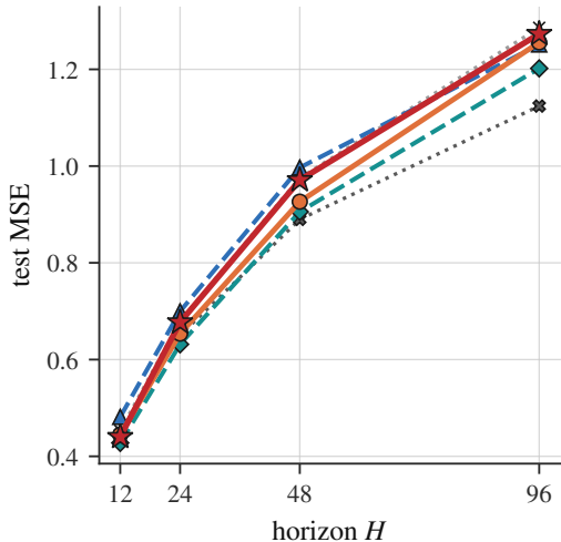
METR-LA traffic
