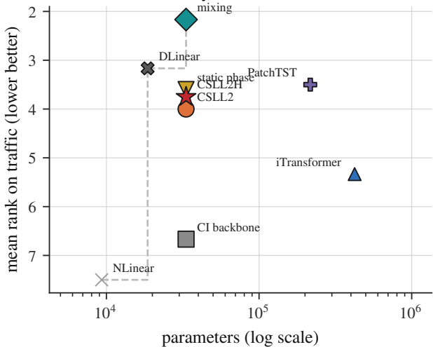
Accuracy vs. cost on traffic
