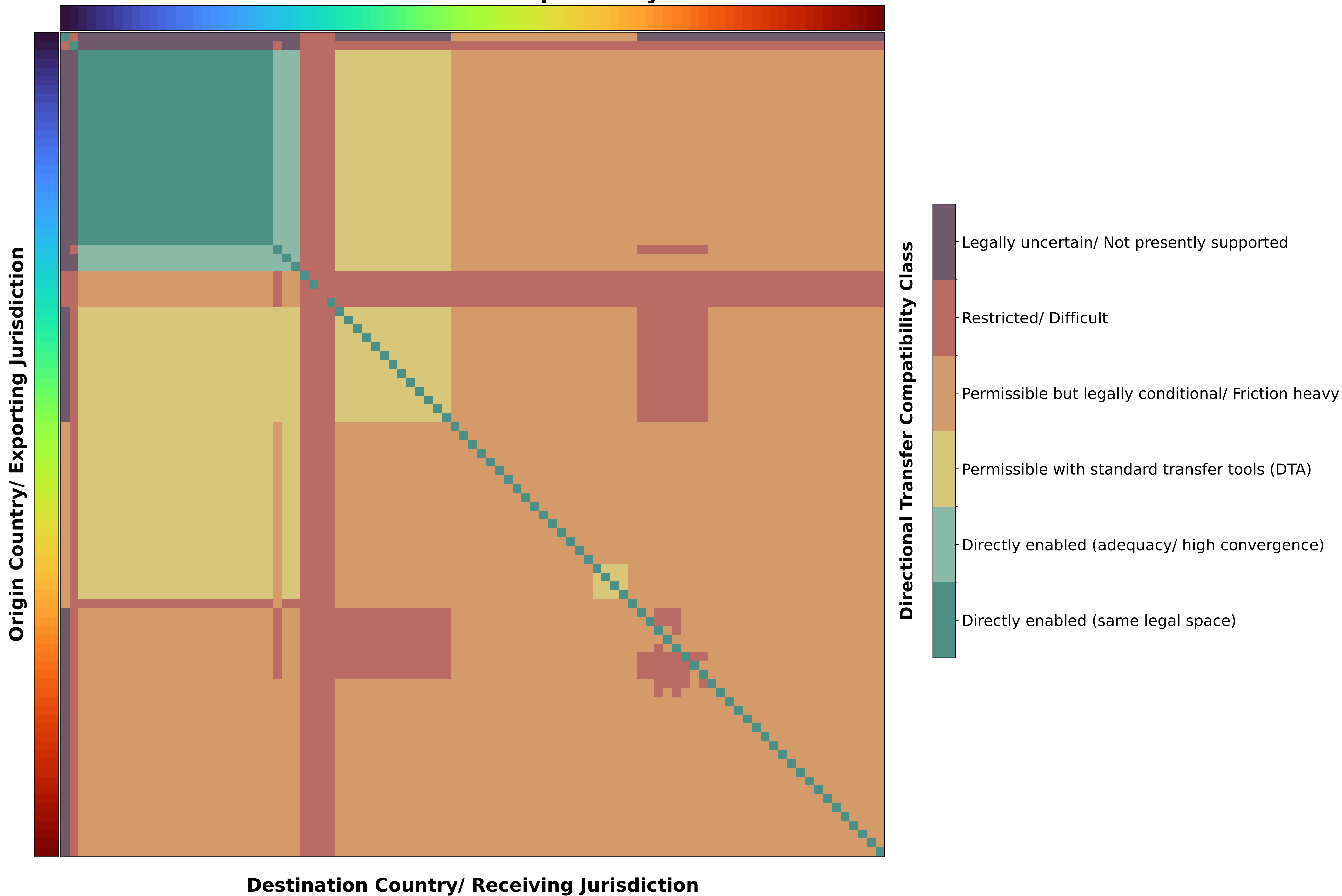
Clustered Directional Compatibility Matrix
