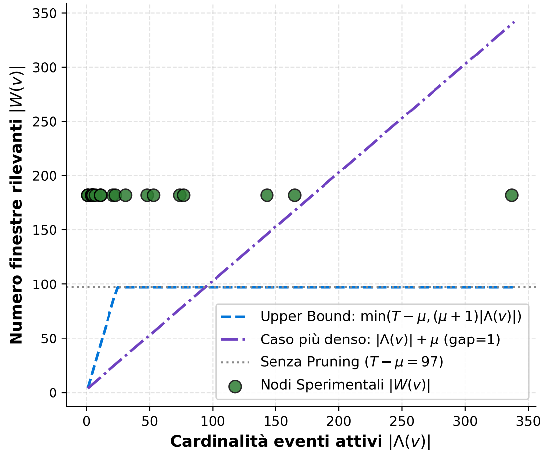
Verifica Bound Teorico |W(v)| vs |\Lambda(v)|
