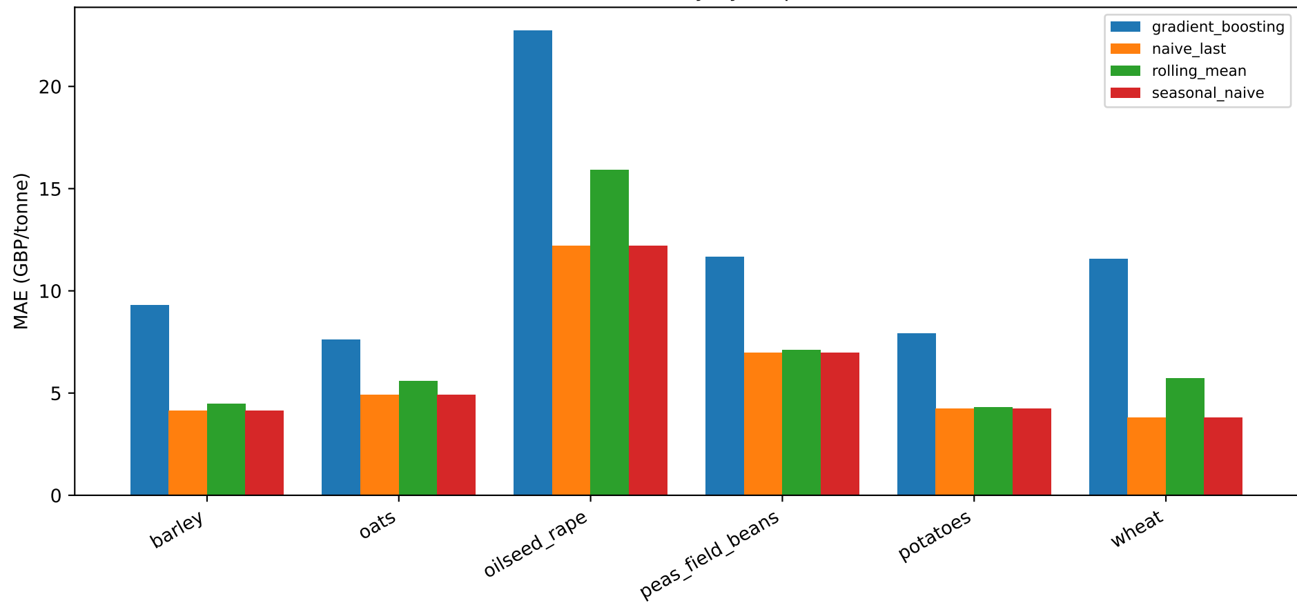
Price forecast accuracy by crop and model
