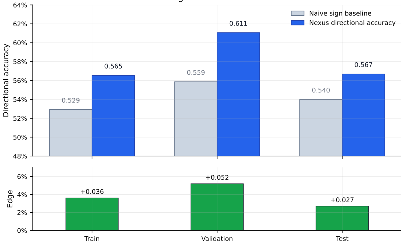
Directional Signal Relative to Naive Baseline
