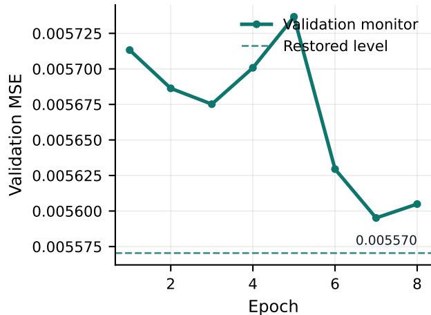
Hard-example validation
