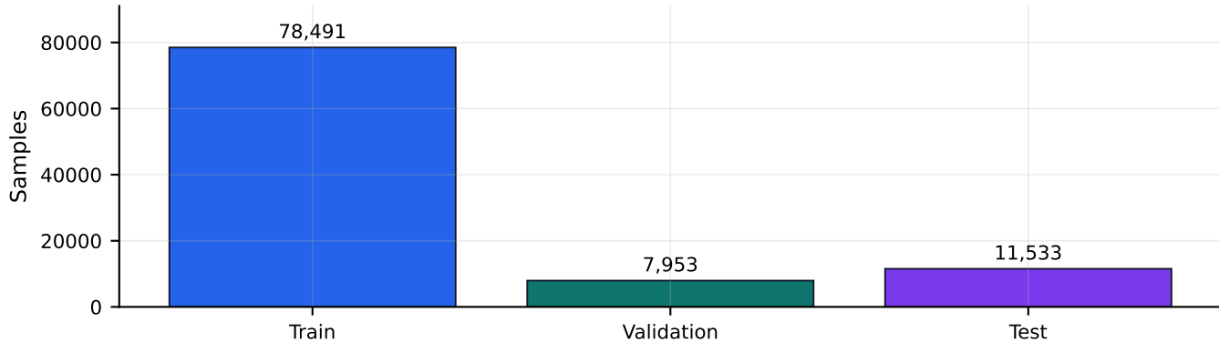
Expanded-Universe Split Scale
